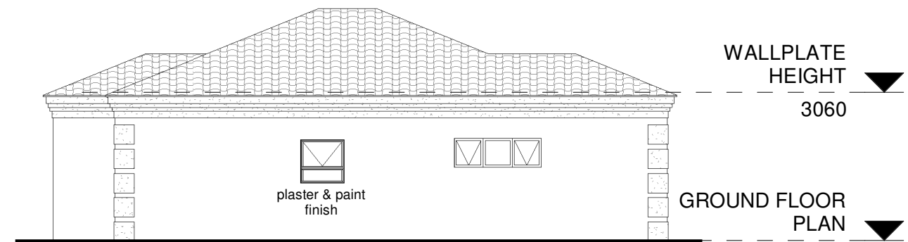
6 WEST ELEVATION 1 : 100
