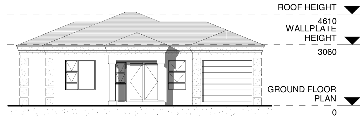
4 SOUTH ELEVATION 1 : 100
