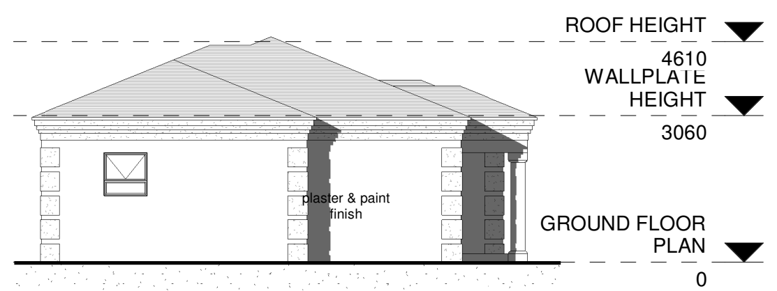
6 WEST ELEVATION 1 : 100
