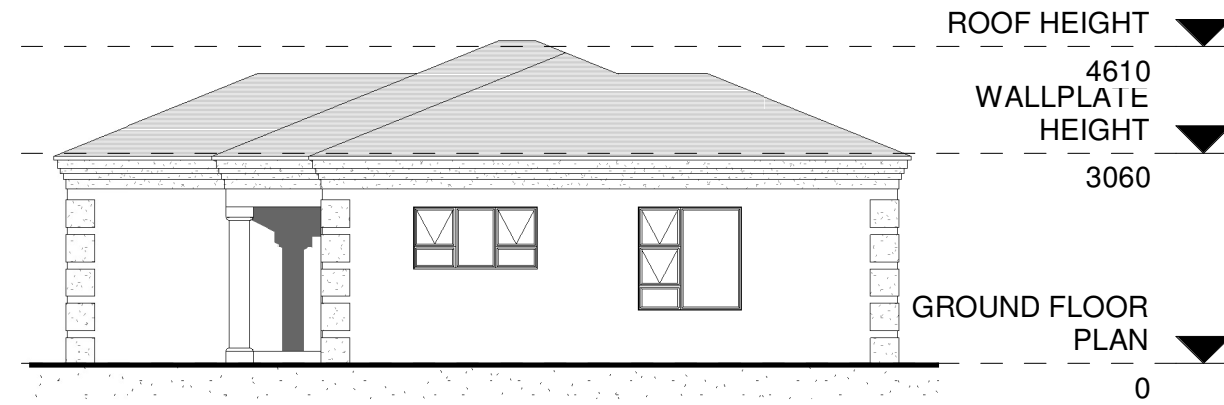
3 NORTH ELEVATION 1 : 100
