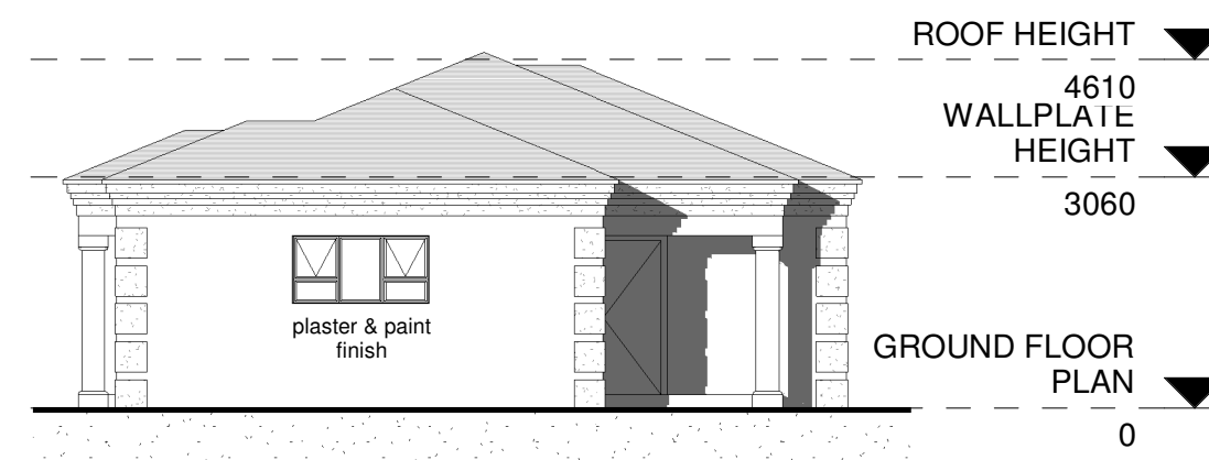
5 EAST ELEVATION 1 : 100
